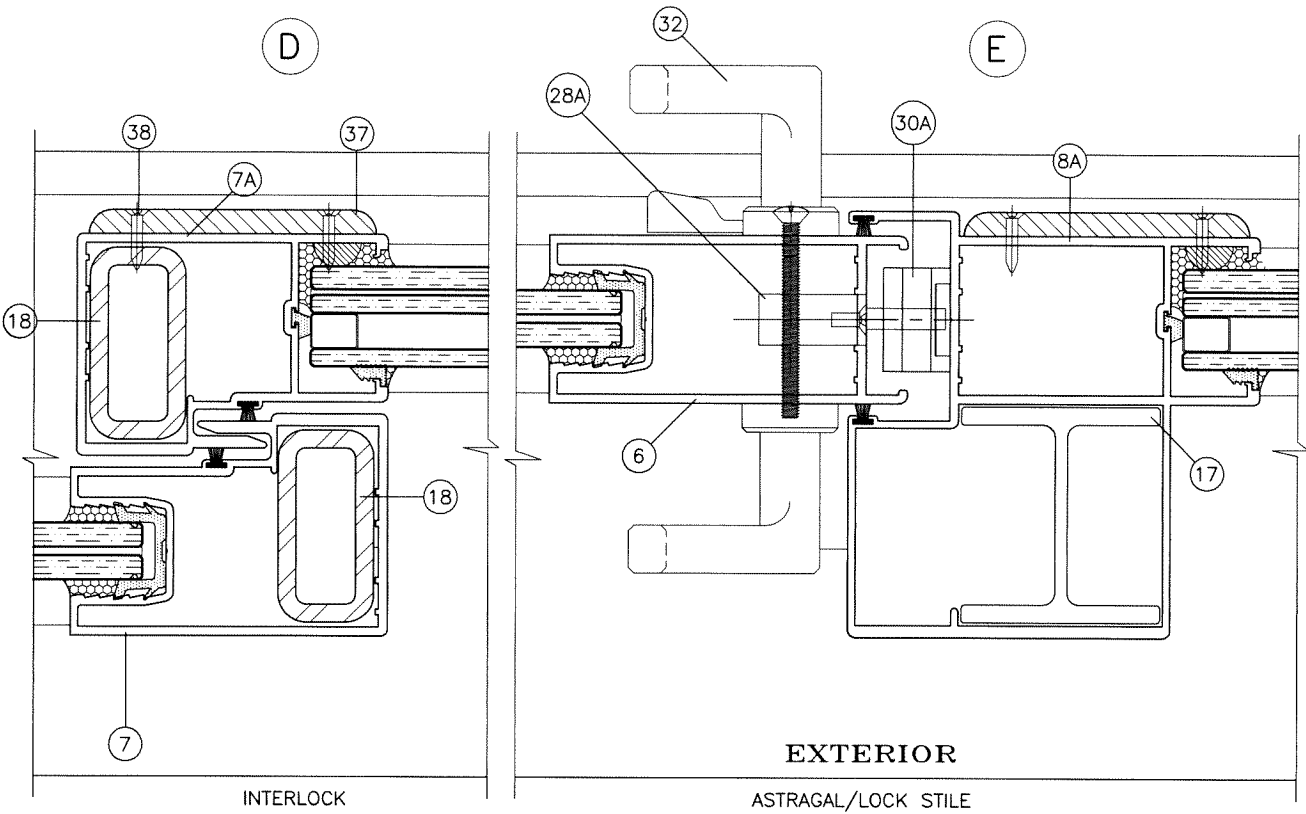
REINFORCING LEVEL '1'
