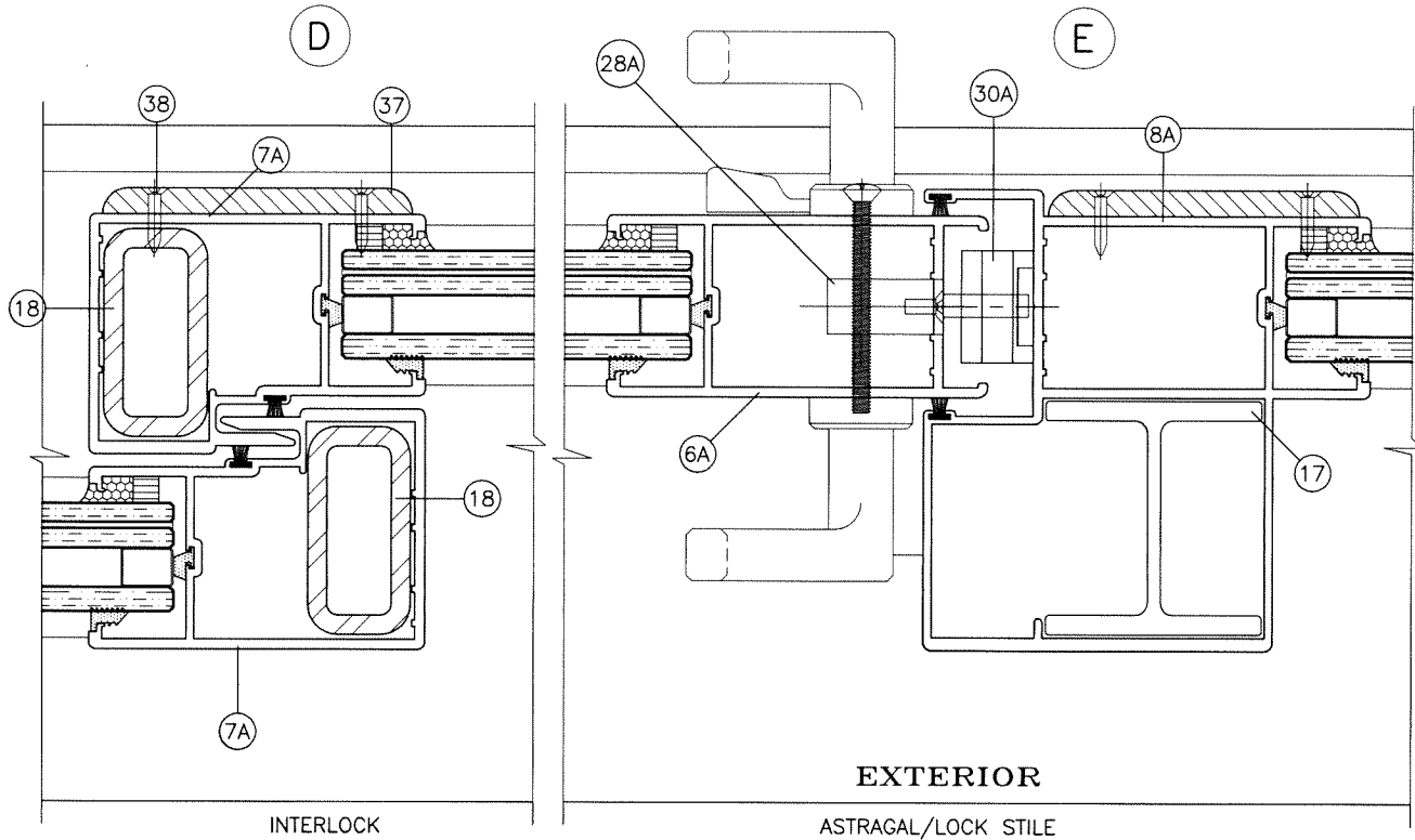
REINFORCING LEVEL '1'
