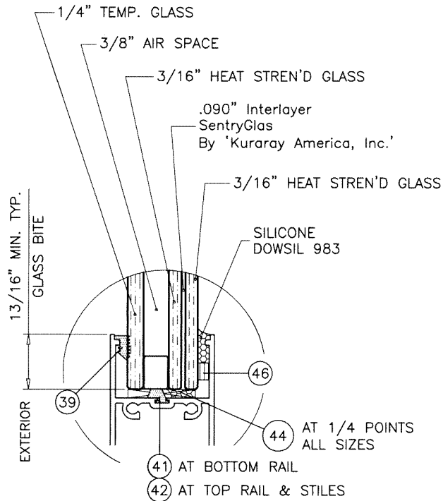
GLASS TYPE 'C' 1-1/16" OVERALL INSUL. LAM. GLASS GLAZING DETAIL
