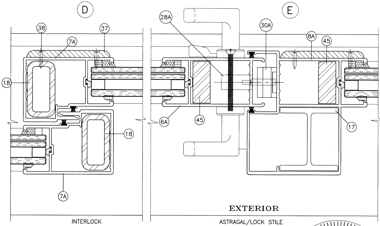
REINFORCING LEVEL '2'
