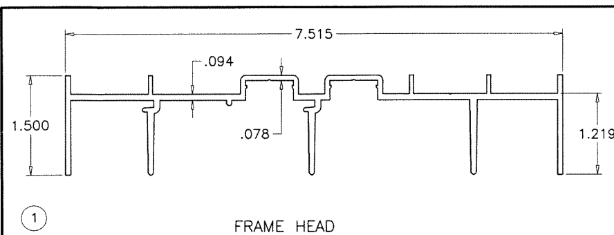
FRAME HEAD
